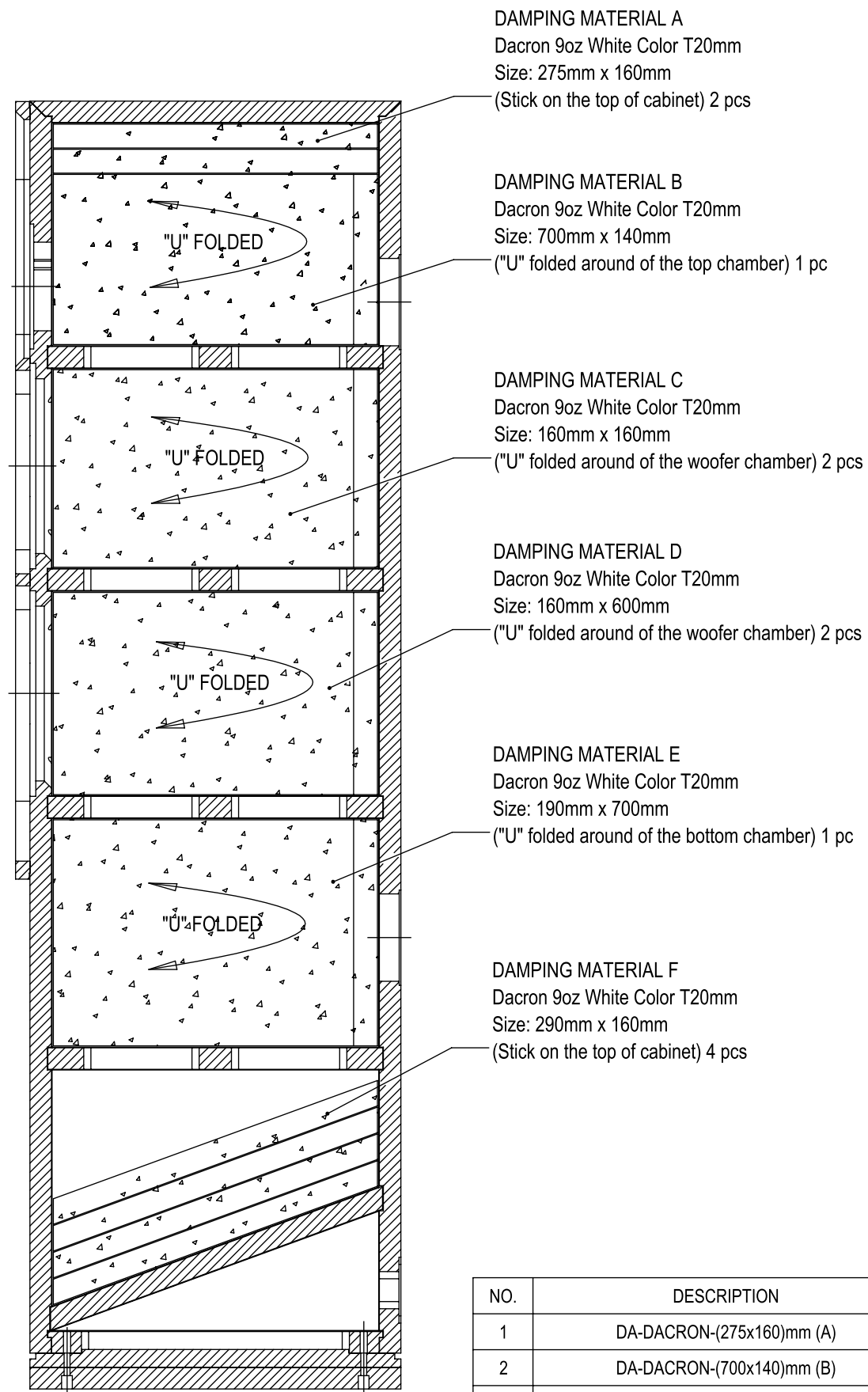
" SECTION VIEW "
