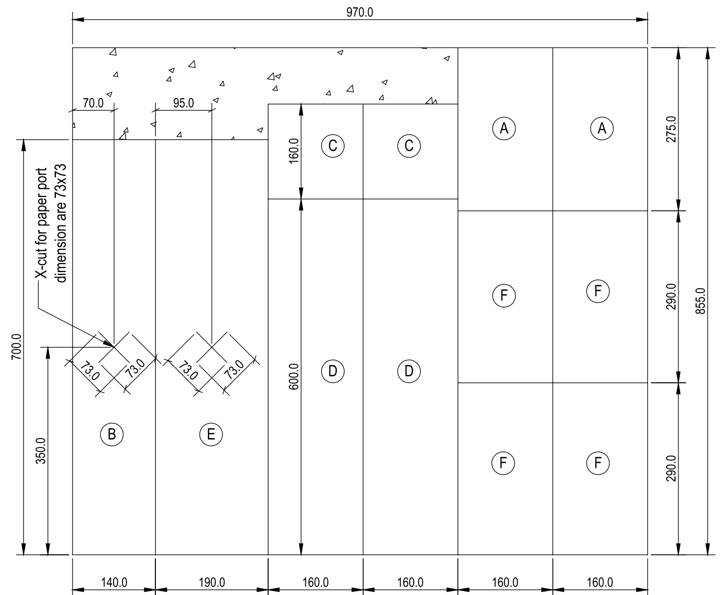
" DAMPING MATERIAL CUT PATTERN "
