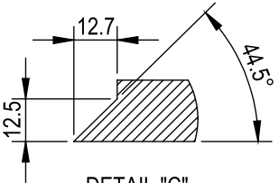
DETAIL "C" SCALE 1 : 2
