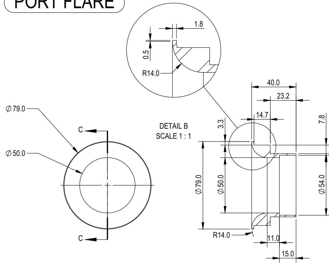
SECTION C-C
